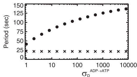
FIG. 5. From the model of Huang et al. (18), the oscillation period versus the nucleotide exchange rate, \sigma_D^{\text{ADP} \rightarrow \text{ATP}} , on a linear-log scale (filled circles) for a 4- \mu\text{m} -long bacterium. The period increases sublogarithmically as the nucleotide exchange rate is increased. Also shown (X's, scaled by a factor of 5) is the average time interval between every binding of MinD to the membrane. This is roughly constant as the nucleotide exchange rate increases, indicating that the period increases because the number of MinD bindings increases.
