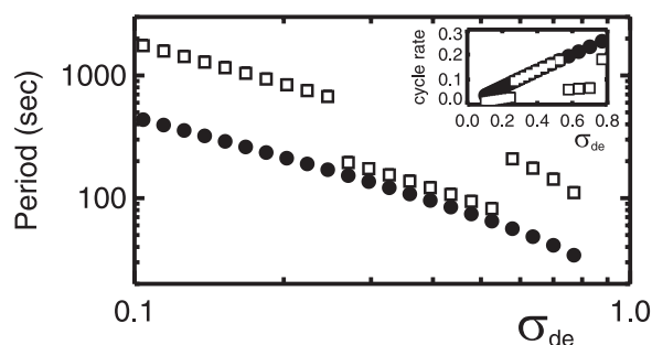
FIG. 6. From the model of Huang et al. (18), the oscillation period versus the MinE-stimulated MinD-ATPase rate, \sigma_{de} , on a log-log scale. Shown are results for a 4- \mu\text{m} -long bacterium and a 10- \mu\text{m} -long bacterium (filled circles and open squares, respectively). A strong decrease of oscillation period with increasing ATPase rate is seen. The longer periods for 10- \mu\text{m} -long bacteria with smaller or larger \sigma_{de} are associated with end-to-end oscillation, while intermediate \sigma_{de} values exhibit a symmetric breathing mode pattern. The inset shows the inverse time between MinD bindings (rebinding rate, in 1/s ) versus \sigma_{de} .
